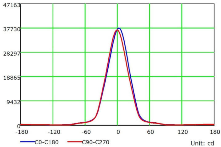
Isocandela (rectangle)
